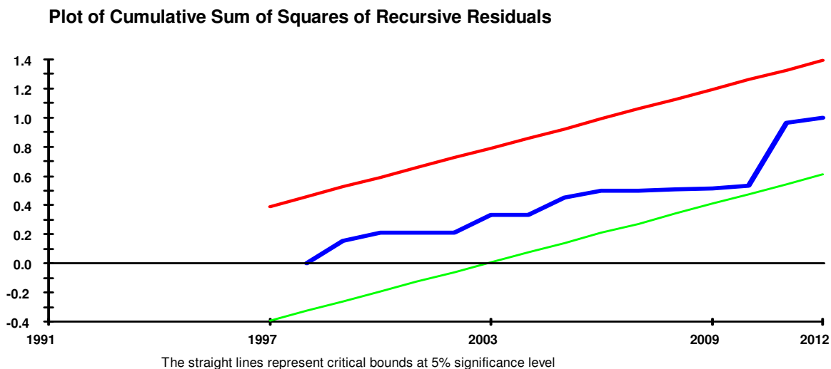
Figure 3B Cumulative Sum of Squares of Recursive Residuals
