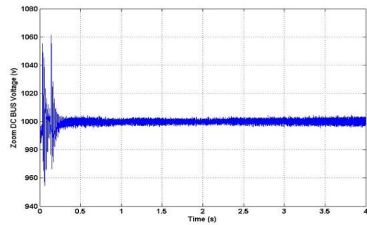
(c) DC bus Voltage
