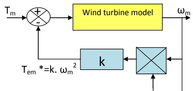
Fig 6 : MPPT control strategy
