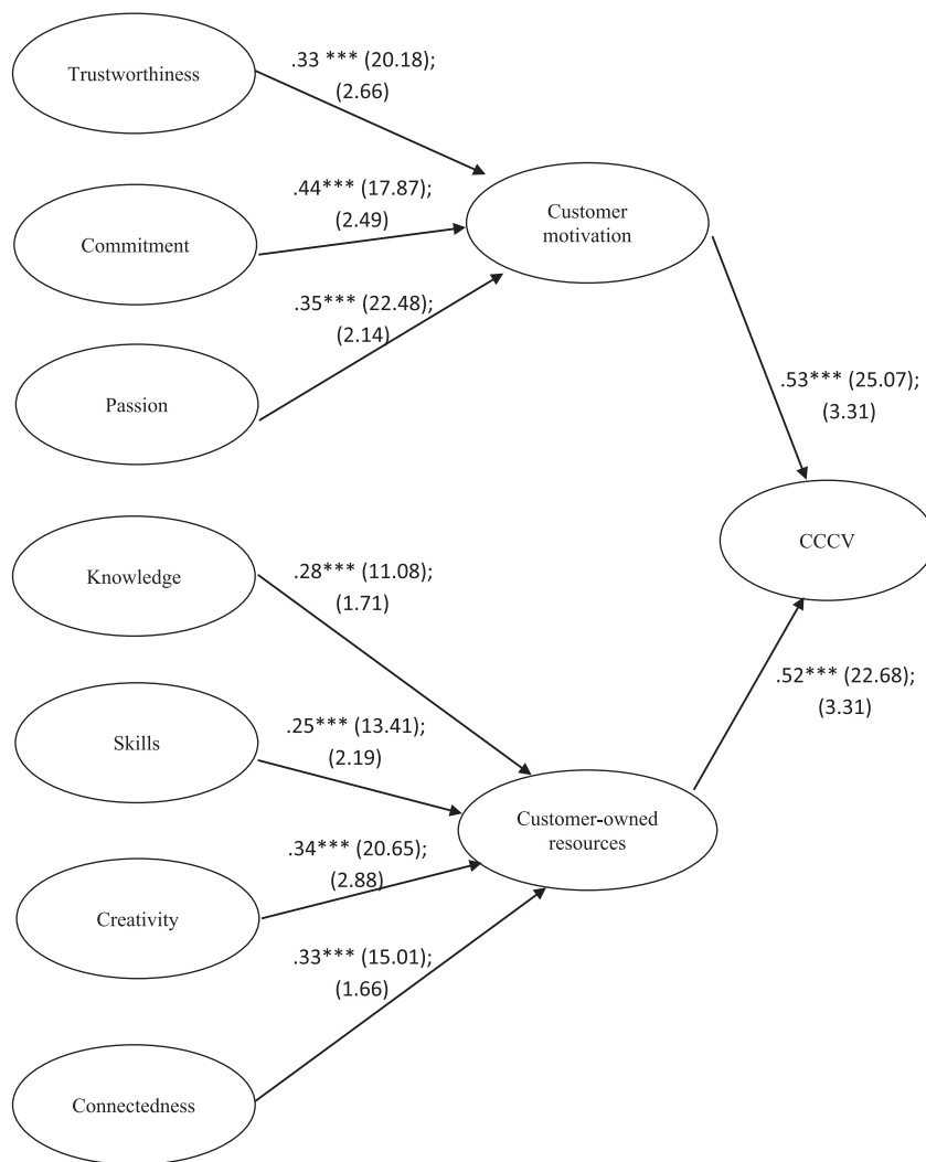
Fig. 1. Results for the third-order model of the CCCV scale. Path coefficients (t-values); (VIF) (Study 5). *** p < .001 .
