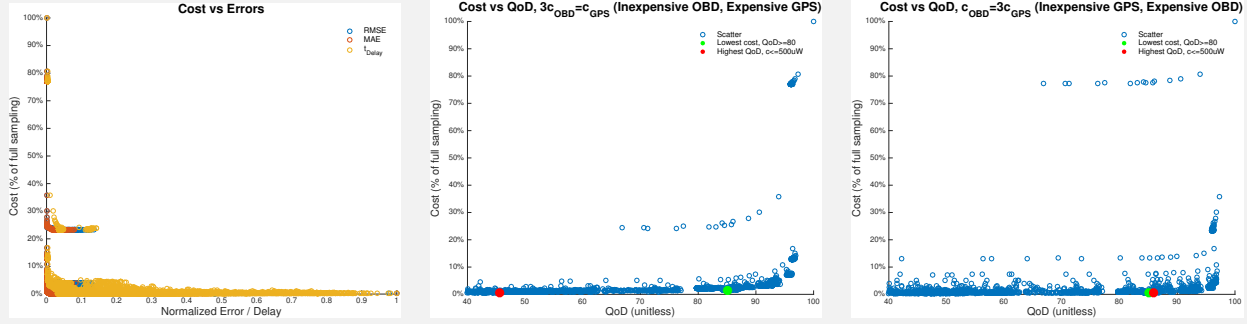
(a) Cost versus normalized RMSE, MAE, and average threshold cross detection delay. (b) Cost versus aggregate QoD; (c) Cost versus aggregate QoD; \lambda_{GPS} = 10\mu W/sample and \lambda_{GPS} = 3.3\mu W/sample and \lambda_{OBD} = 3.3\mu W/sample . Lowest \lambda_{OBD} = 10\mu W/sample ; lowest error for cost for error target in green; lowest error target cost in red. for target cost in red.
