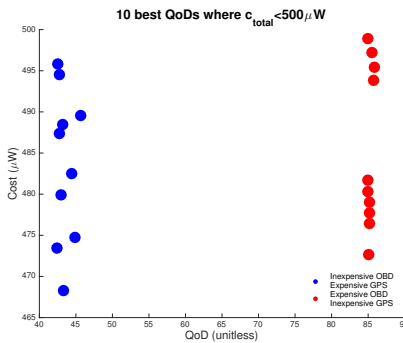
Fig. 7: The ten best QoDs meeting c_{total} < 500\mu W are shown for the case where \lambda_{OBD} = 3\lambda_{GPS} and 3\lambda_{OBD} = \lambda_{GPS} . Note that when GPS is relatively less expensive, it is sampled more frequently – dramatically increasing the QoD.
