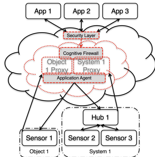
Fig. 2: This architecture builds upon the cloud connectivity approach, adding elements to improve efficiency, privacy, and security.
