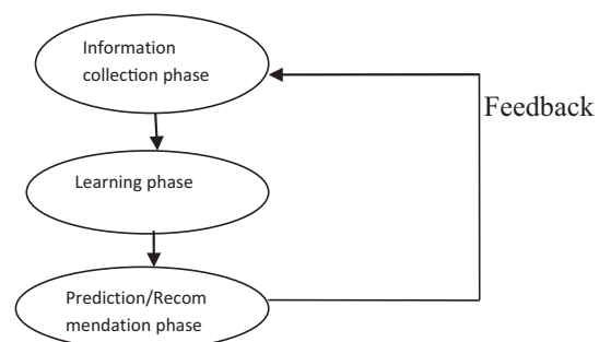
Figure 1 Recommendation phases.
