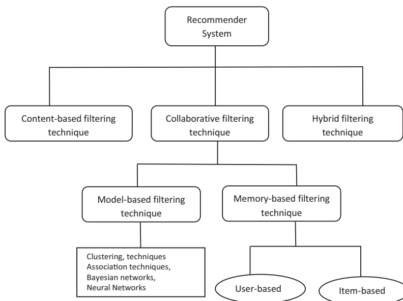
Figure 2 Recommendation techniques.
