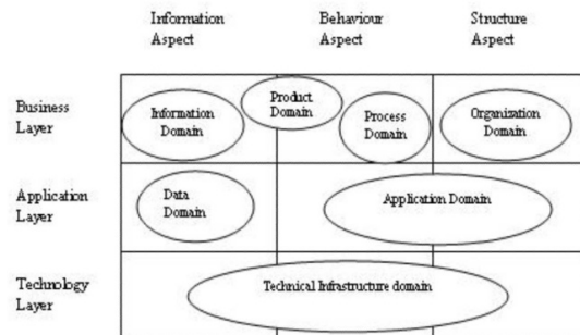
Figure 1. ArchiMate Framework [14]
