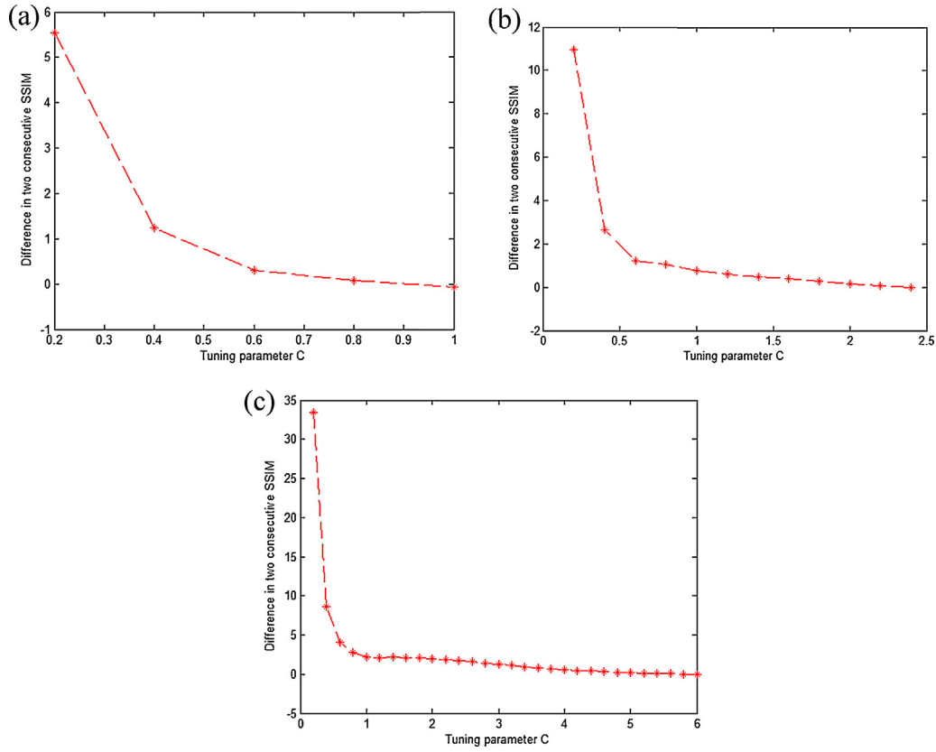
Fig. 3. Relative difference of SSIM for Lena image. (a)–(c) Relative difference of SSIM with noise standard deviation 0.4, 0.7 and 1 respectively.
