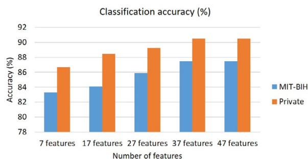
Fig. 10. Classification accuracy of the proposed framework.
