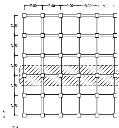
Figure-1: Configuration plan of 8-storey Building at below storeys
