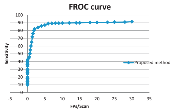
Fig. 8 – FROC curve.
