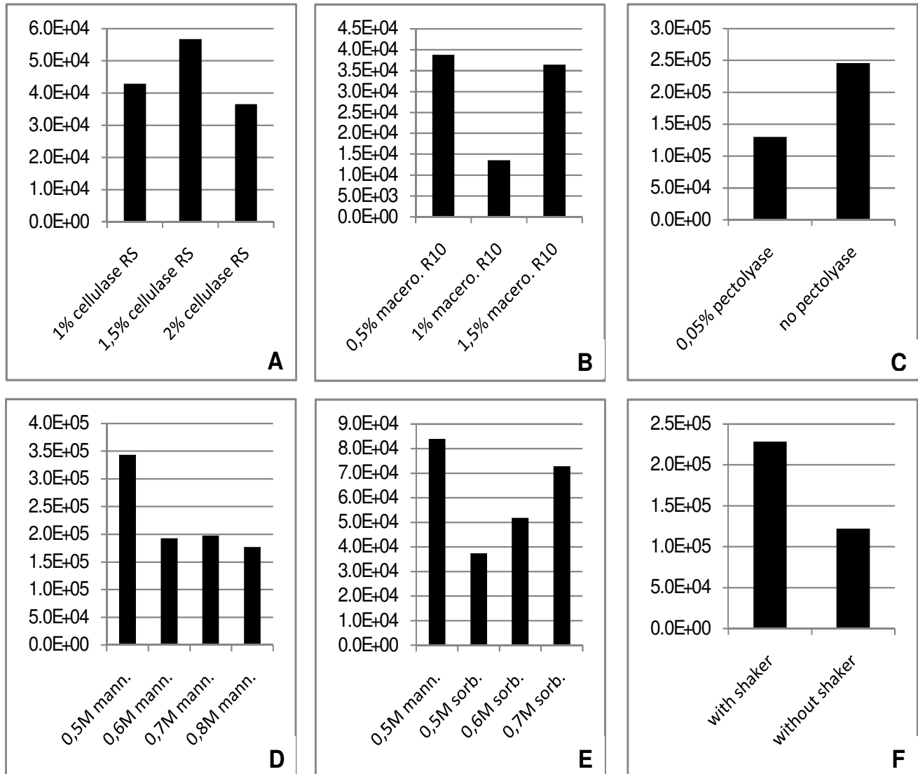
Figure 1. Preliminary tests to determine the optimal enzyme mixture. The basic mixture consisted of 2% cellulase RS, 0.5% macerozyme R-10 and 0.5M mannitol. In 6 independent tests (a) the cellulase concentration, (b) the macerozyme concentration, (c) the pectolyase concentration and (d) the mannitol concentration was varied. (e) Sorbitol was used as an osmoprotectant in different concentrations and (f) shaking during incubation in the enzyme mixture was beneficial.
