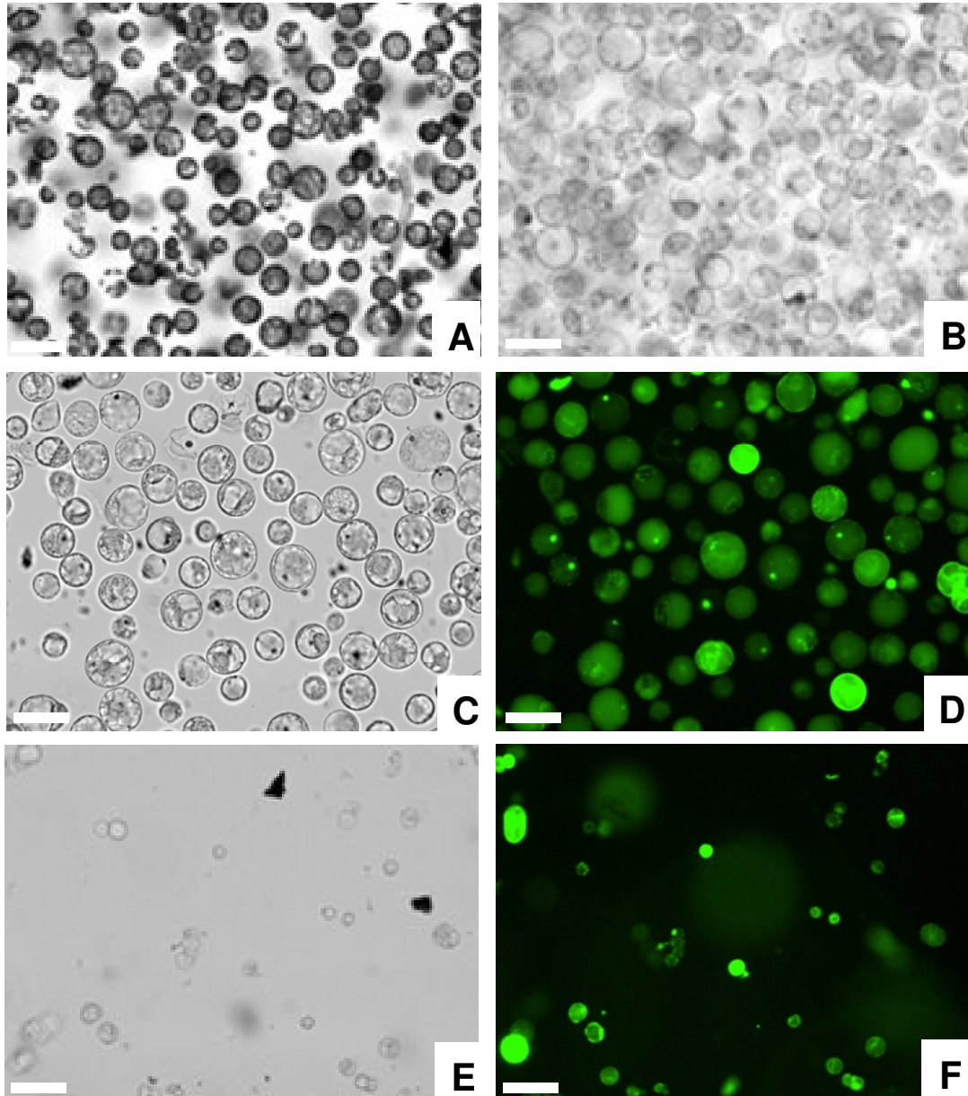
Figure 3. Protoplasts isolated from different types of tissue culture material. (a) Protoplasts from leaves of in vitro plants. (b) Protoplasts from callus induced on leaves. (c – d) Protoplasts from callus induced on transgenic hairy roots showing GFP fluorescence. (e – f) Protoplasts from transgenic hairy roots pretreated with IBA, also with GFP fluorescence. Scale bars are 50 \mu\text{m} .
