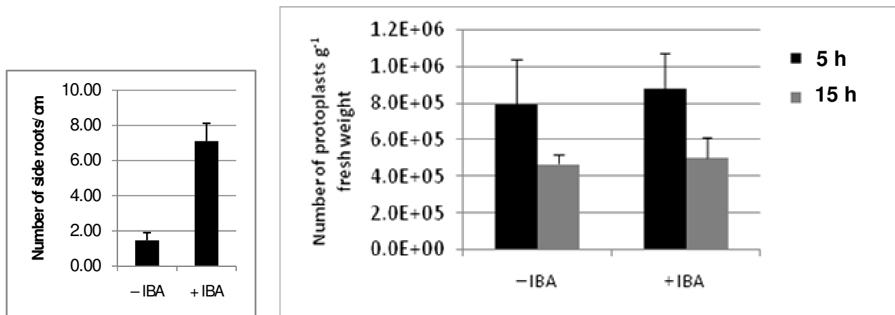
Figure 2. Effect of IBA treatment (a) on lateral root formation and (b) on protoplast yield, protoplast isolation tested for two incubation times, 5 and 15 hours. Results are mean values of three independent repeats.
