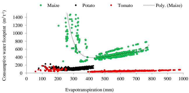
Figure 3. The resultant ET and consumptive WF for all experiments: different management practices for all cases. The dotted line is a polynomial fit to data points for maize.
