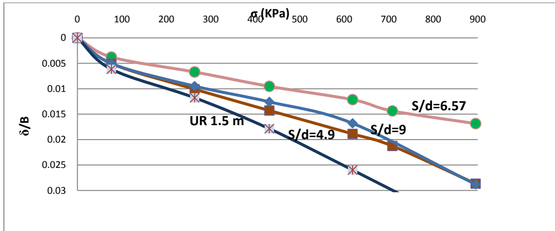
Fig. 6 The effect of s/d ratio on the load settlement curve for non-connected pile raft system, using a granular layer with an optimum thickness of 1.5m
