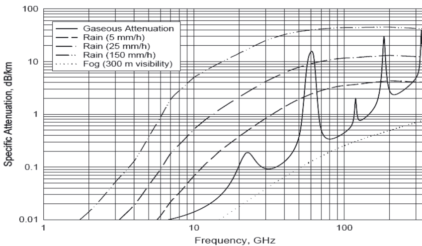
Fig. 6. Atmospheric attenuation versus frequency.
