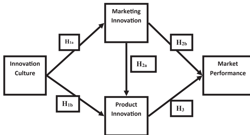
Fig. 1. Research framework.
