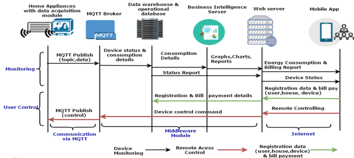
Fig. 2. Sequence Diagram
