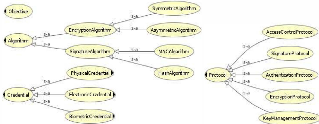
Figure 2: Security ontology.
