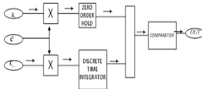
Figure 11. Schematic Diagram of PI Controller
