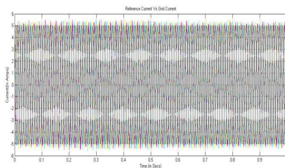
Figure 26. Reference Current &amp; Grid Current
