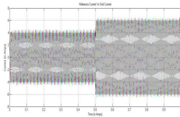
Figure 18. Reference Current &amp; Grid Current
