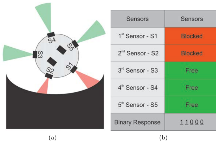
Figure 2: Proposed encoding.
