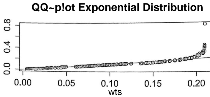
Figure 2. QQ-plo( for Exponential Distribution for 20 nodes with CSMA protocol, sending 1 packet/1 second
