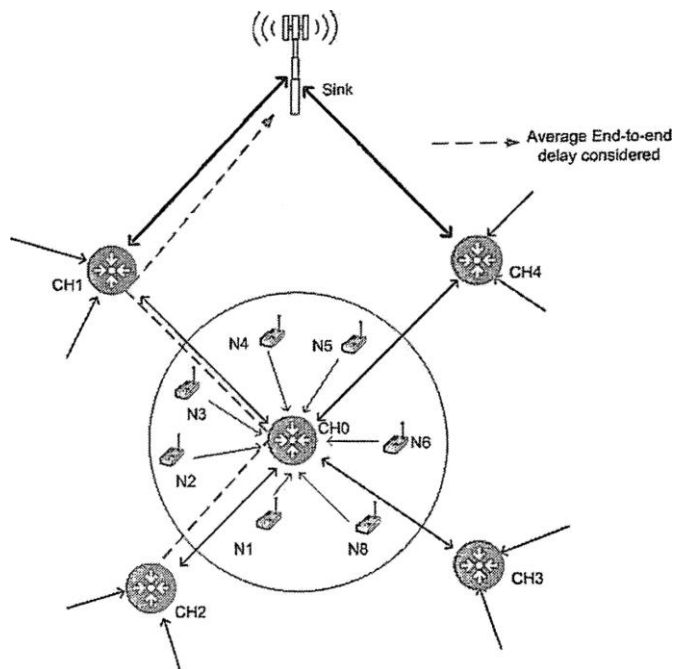
Figure 1: Network topology of the reference scenario
