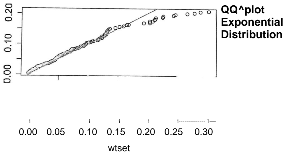
Figure 3: QQ-plot for Exponential Distribution for 10 nodes with CSMA, sending 1 packet/10 minutes
