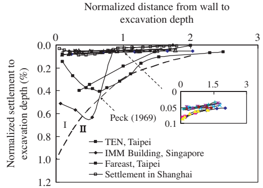
Figure 8. Distribution of the ground surface settlement normalized by the excavation depth.
