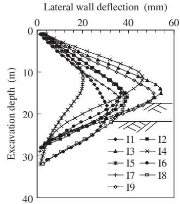
Figure 4. Maximum lateral wall deflection at the final excavation depth.
