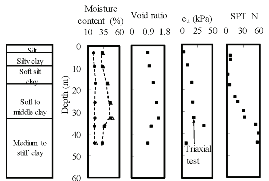
Figure 3. A typical soil profile and soil parameters.
