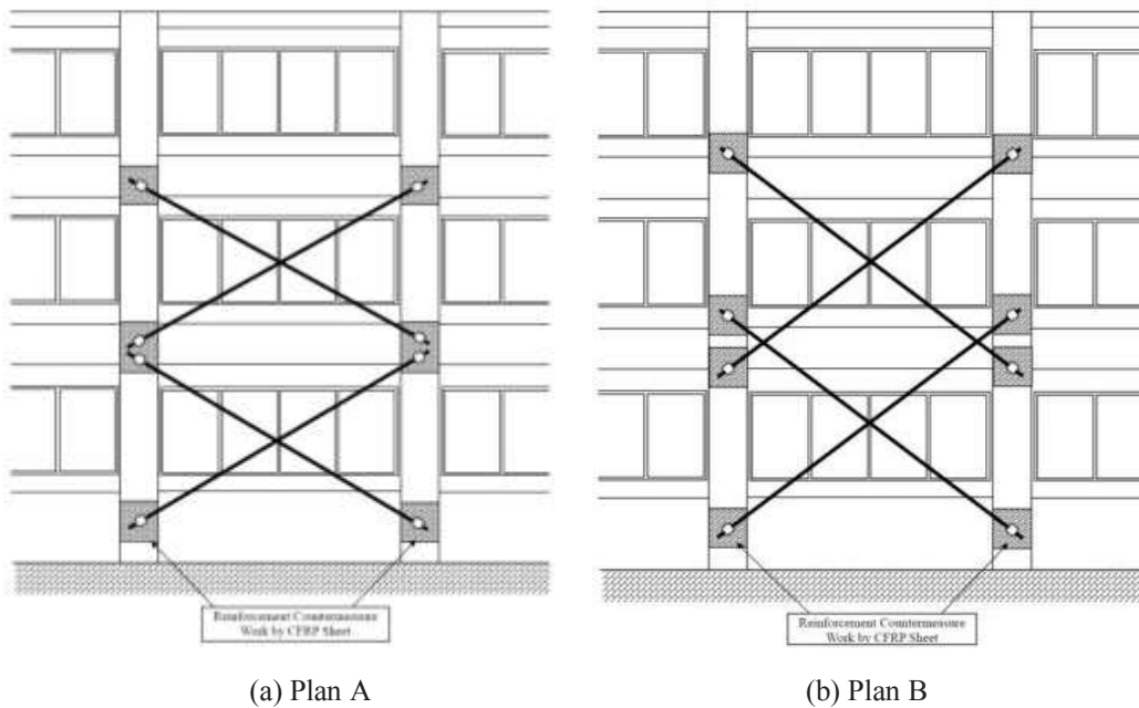
Figure 8. Elevation view of RC building with the ACM brace
