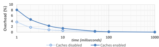
Fig. 3. Correlation between guest-switching rate and performance overhead
