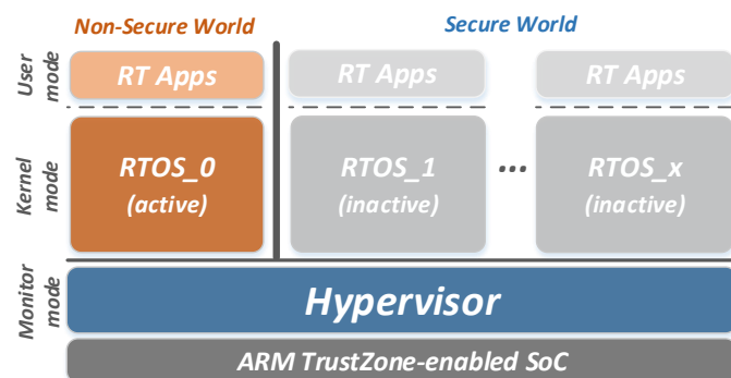
Fig. 1. TrustZone-assisted Virtualization Architecture
