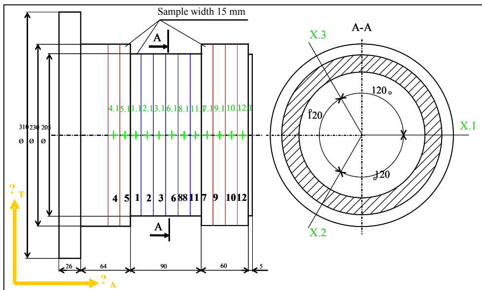
Fig.1. Simplified schematic view of production order (turning) of individual samples and analyzed network representation of the selected points marked with lines of residual stress determination.
