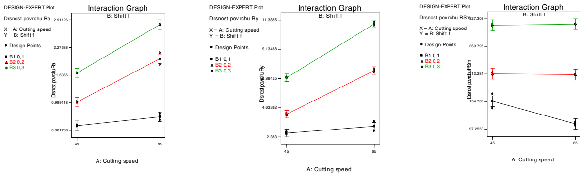
Fig. 7. Interaction graph of parameters Ra, Rz and Rsm.
