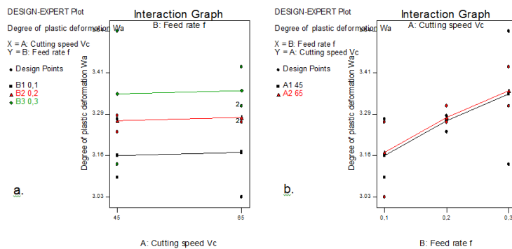
Fig. 4. Interaction graphs for degree of deformation in axial direction.
