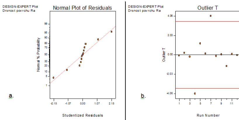
Fig. 6. Model tests for Ra parameter: a) Normal probability plot of residuals, b) Outlier test.
