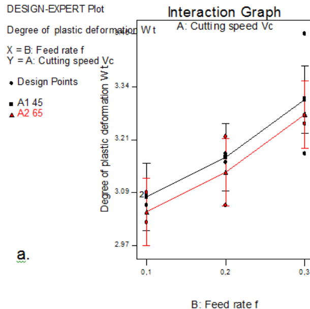
Fig. 5. Individual Values of degree of deformation in tangential direction.
